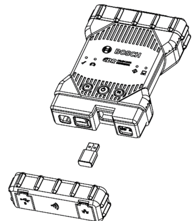
Figure 2 Insert Wireless USB Dongle
